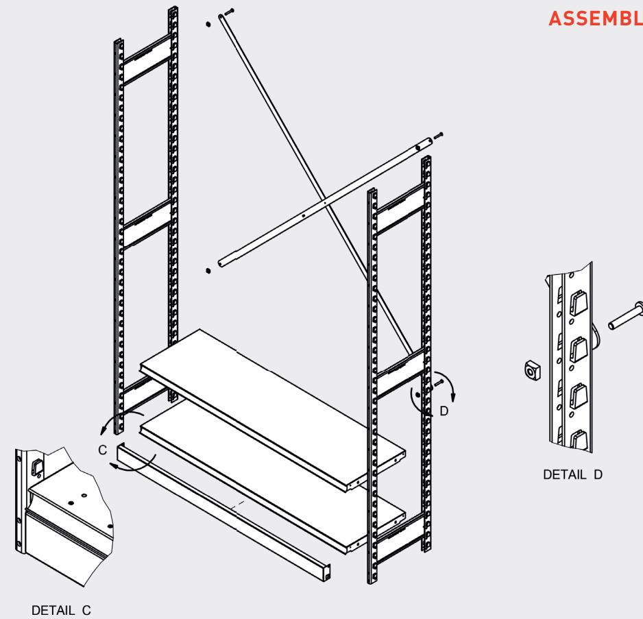
DETAIL C
