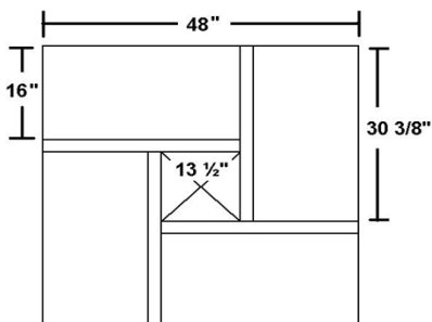
16" x 30" shelf max.
