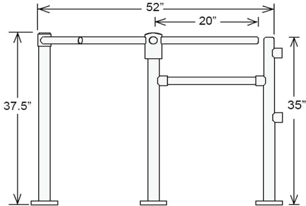
TOURNIQUETENT Four-arm turnstile model T chrome finished
