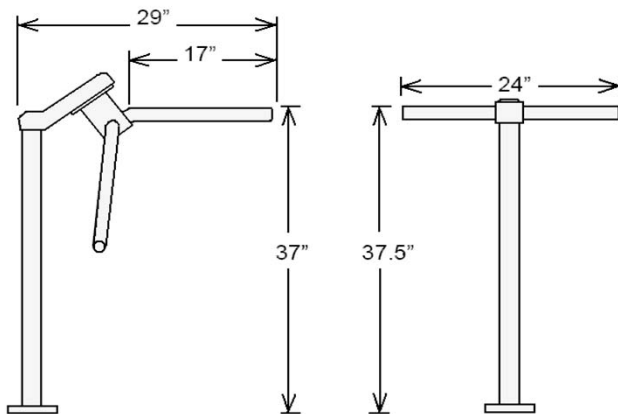
TOURNIQUETW Three-arm turnstile model W chrome finished
