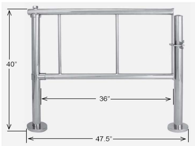
PORTEHANDICAP48 LG manual closing gate, 48" wide with manual latch, chrome finished
