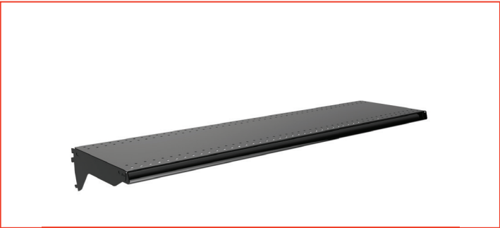
ITEM SLOPED SHELF LENGTH 6" - 8" - 10" - 12" - 14" - 16" - 18" (DEPTH) LENGTH 24" - 48" (IN INCREMENTS OF 6")
