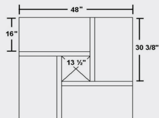
16" X 30" SHELF MAX.
