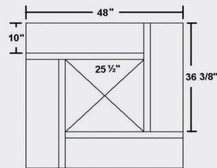
10" X 36" SHELF MAX.
